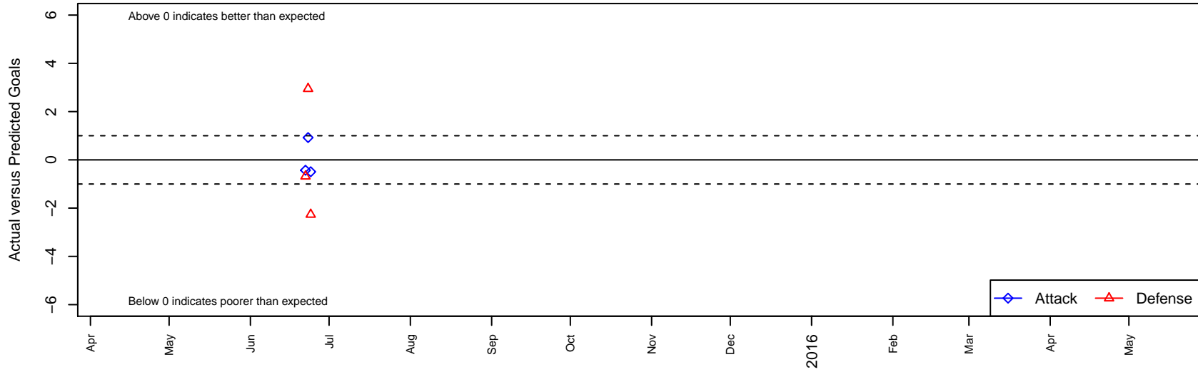
Santa Barbara SC G97 Dots are actual minus expected GF (blue circles) and GA (red triangles). Blue line is smoothed change in attack strength. Red is smoothed change in defense strength.
